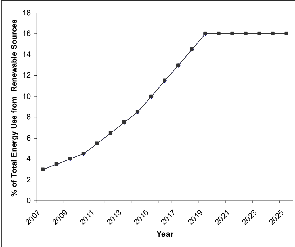
Figure 8.4. Renewable energy targets under the Rhode Island Renewable Energy Standard, 2007-2020.
