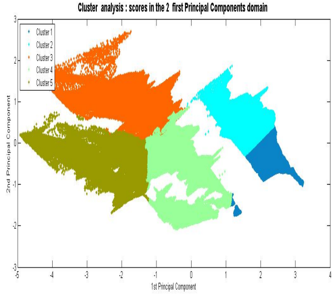
Figure 9 Identification of clusters using the first two principal components for the RI SAMP study area. Cluster definitions, in terms of the input variables, are given in Table 3.
