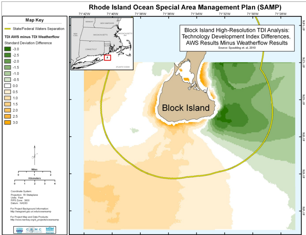
Figure 8 Differential non dimensional TDI for Block Island study area; results from AWS based estimates (Figure 6) minus those from the WIS 101 wind rose (WeatherFlow) estimates (Figure 7).
