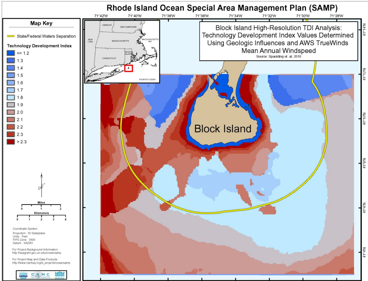
Figure 6 Non dimensional TDI for Block Island Study area with geology using AWS TrueWinds mean annual winds (Brower, 2007).
