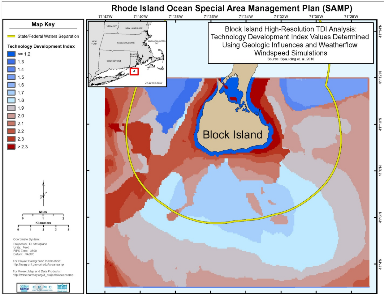
Figure 7 Non dimensional TDI for Block Island Study area with geology with model scaled winds based on WIS 101 wind rose.
