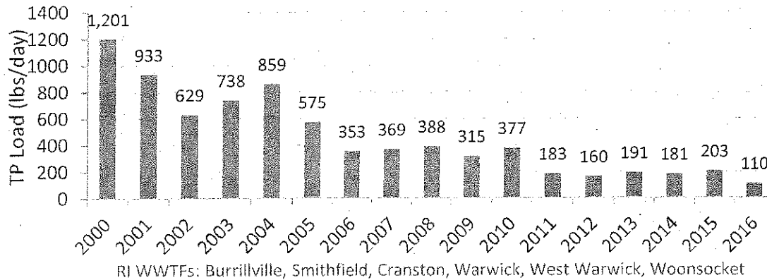
Annual Total Phosphorus Loads - RI "6" WWTFs
