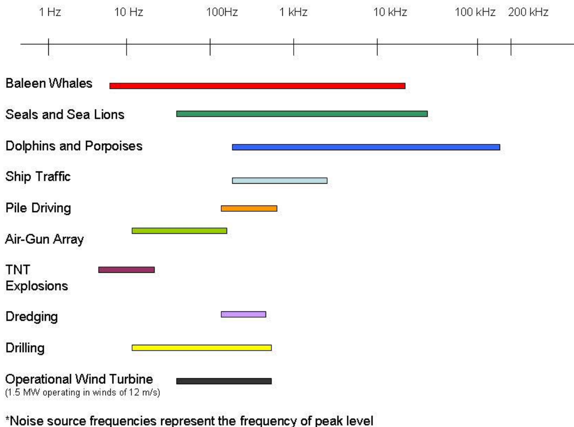
Figure 8.45. Typical frequency bands of sounds produced by marine mammals compared with the main frequencies associated with offshore renewable energy development (OSPAR 2009a).
