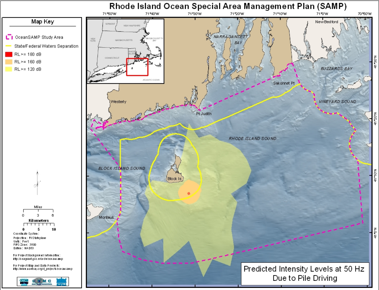
Figure 8.47. Estimate of the affected area in the vicinity of pile driving (Miller et al. 2010).
