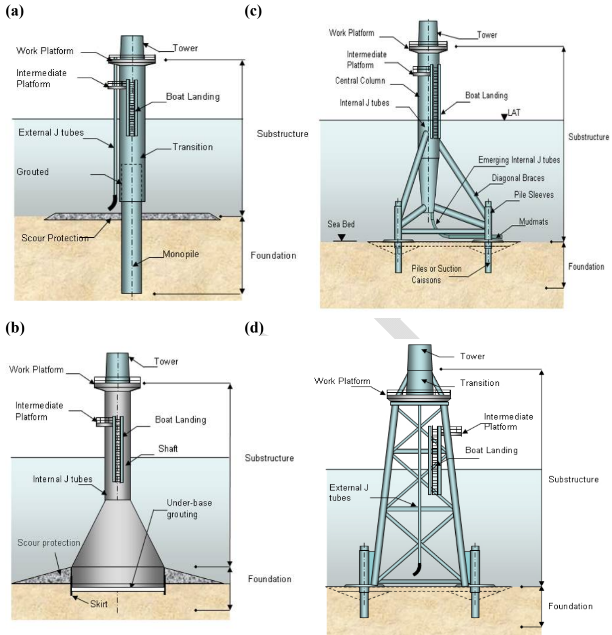
Figure 8.15. Different support structure types for offshore wind turbines (a) monopile, (b) gravity base, (c) tripod, and (d) jacket. (European Wind Energy Association 2009a).
