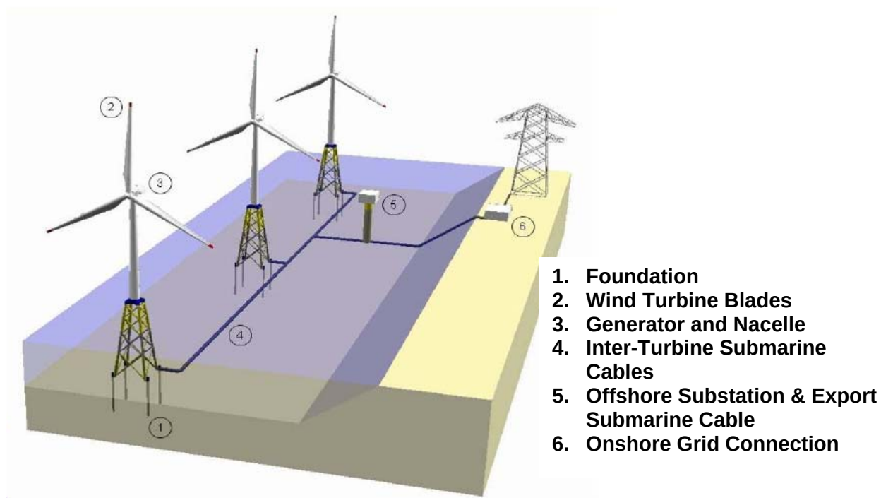
Figure 8.13. Components of an offshore wind facility (Deepwater Wind 2009).
