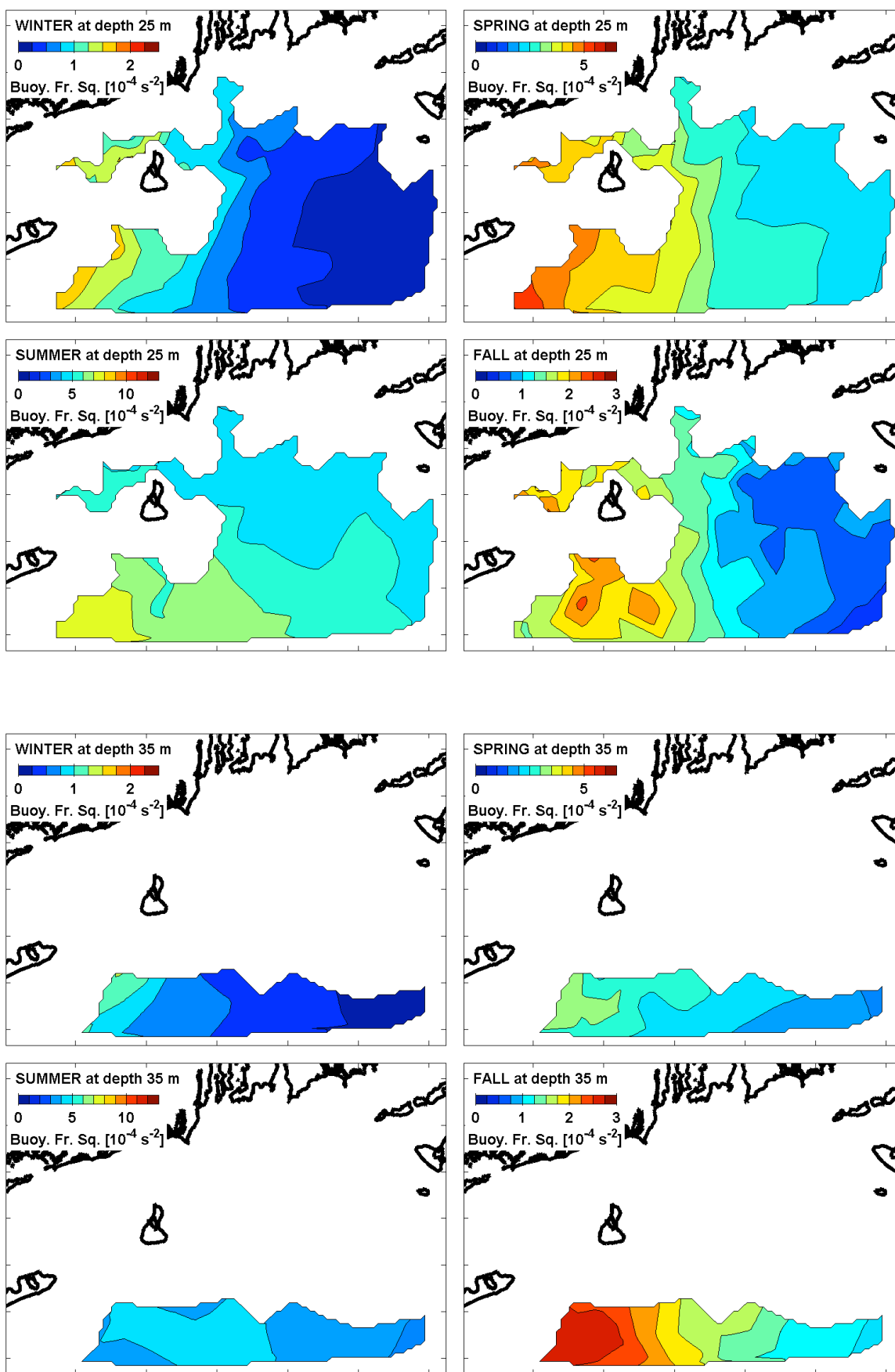
Figure 31. Hydrographic climatology. Stratification. (upper) Depth 25 m. (lower) Depth 35 m.
