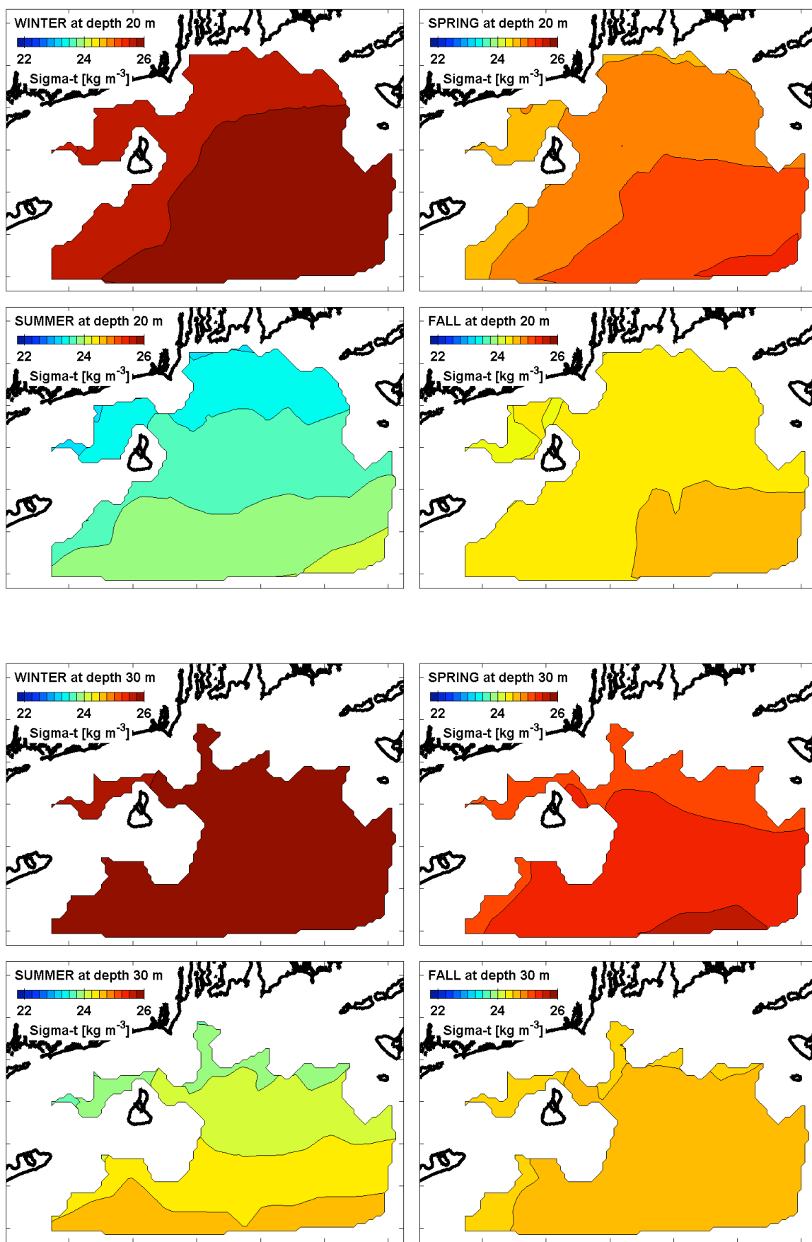
Figure 24. Hydrographic climatology. Density anomaly. (upper) Depth 20 m. (lower) Depth 30 m.
